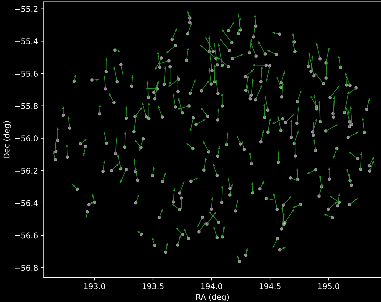
GALAH DR4 Cluster 4 Proper Motion Vectors (n=209)
