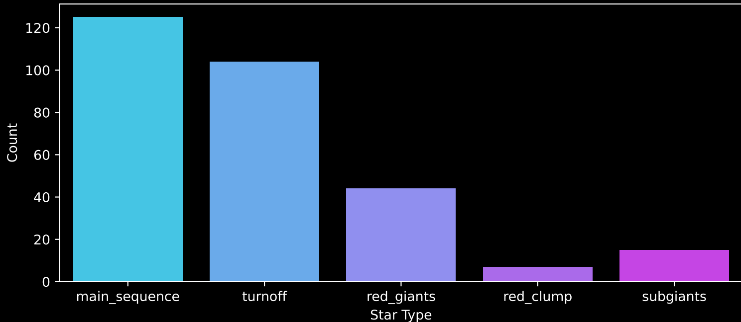
GALAH DR4 Field: [1179] Count plot of Star Type
