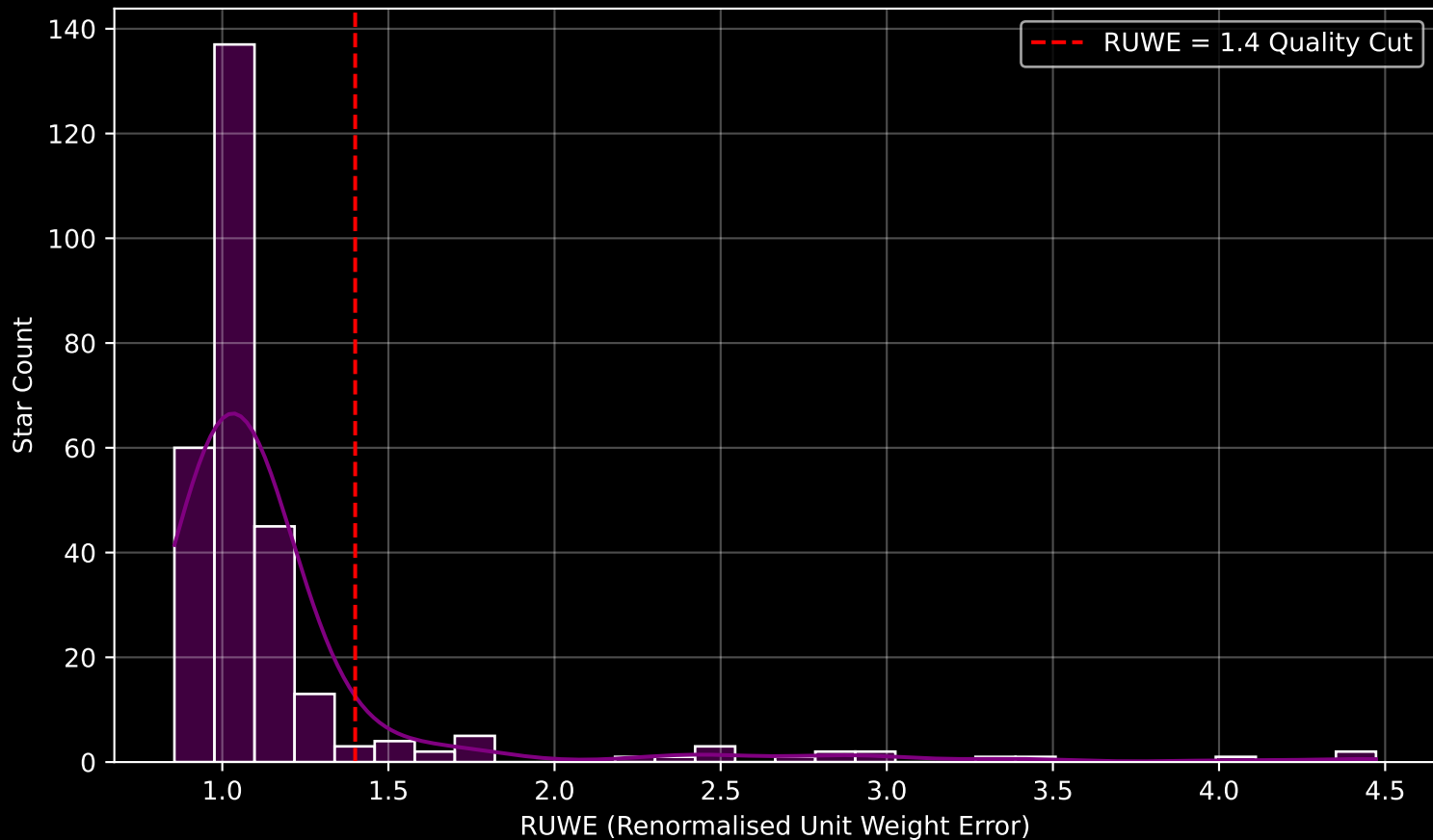
GALAH DR4 Field [1179] RUWE Distribution (n= 284)
