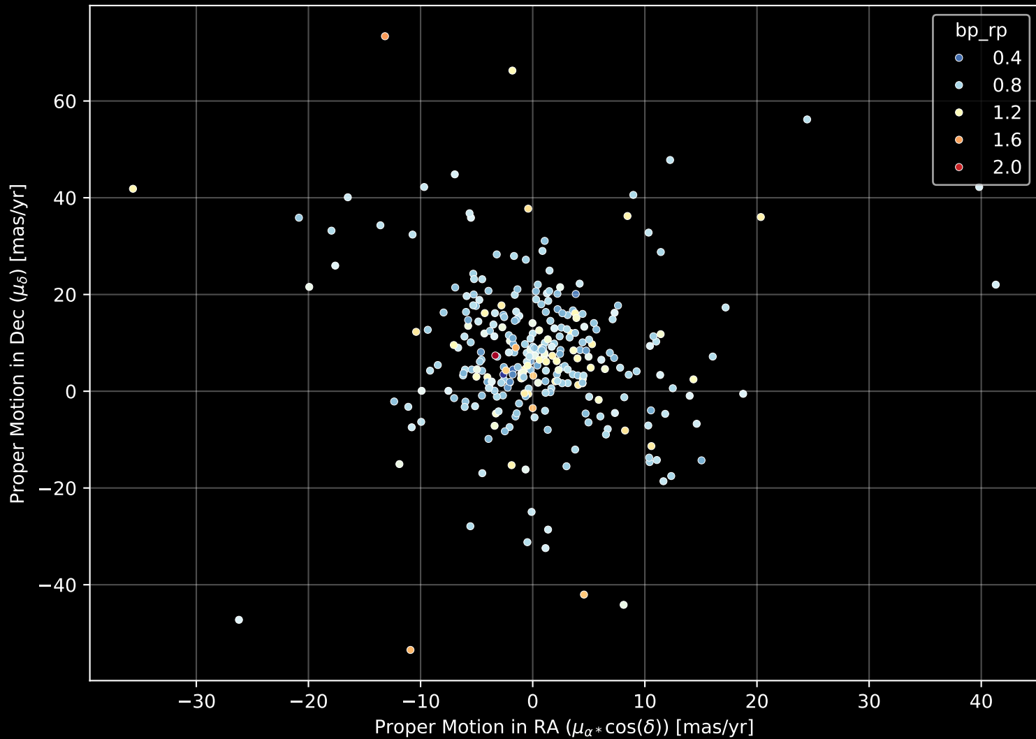
GALAH DR4 Field: [1179] Proper Motion Diagram (n= 295)
